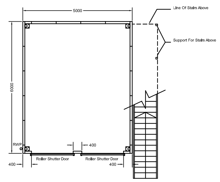
PLANT ROOM PLAN
