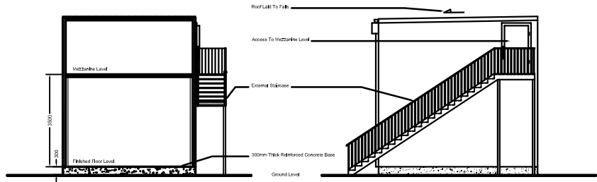
SIDE ELEVATION (SHOWING STAIRCASE)
