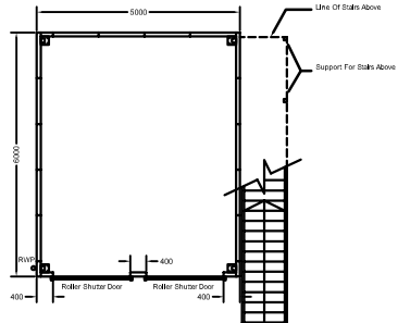
PLANT ROOM PLAN
